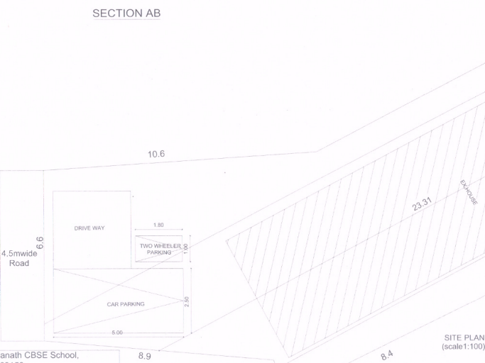
SECTION AB
