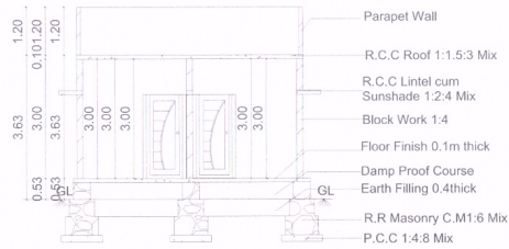
SECTION AB
