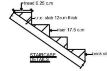
STAIRCASE DETAILS
