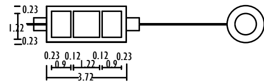
PLAN SEPTIC TANK DETAILS SCALE 1cm : 1m
