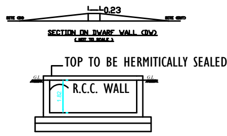
RWH SECTION (SAMPLE)
