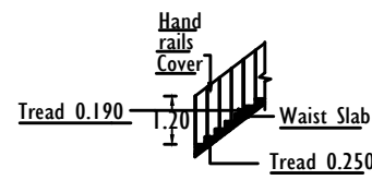
STAIRCASE DETAILS
