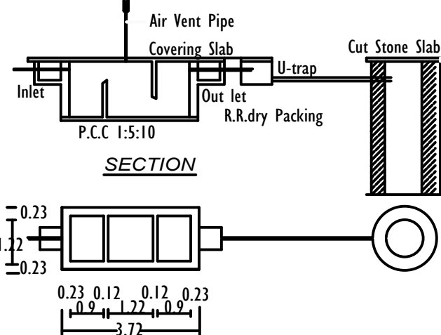
SEPTIC TANK DETAILS SCALE 1cm : 1m
