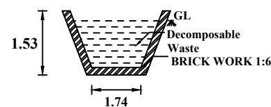
WASTE PIT
