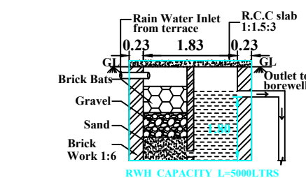
RAIN WATER HARVESTING - PIT
