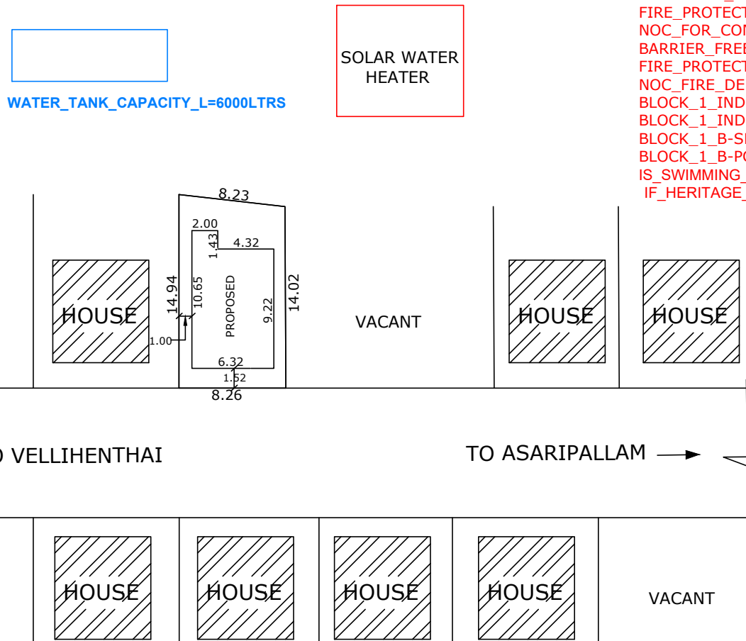
KEY PLAN [SCALE 1:400]
