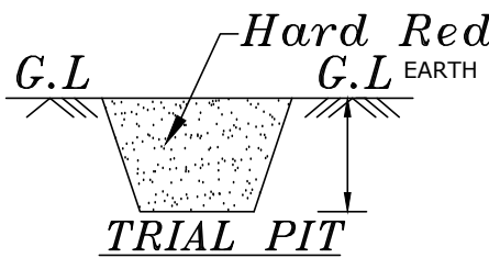
TRIAL PIT
