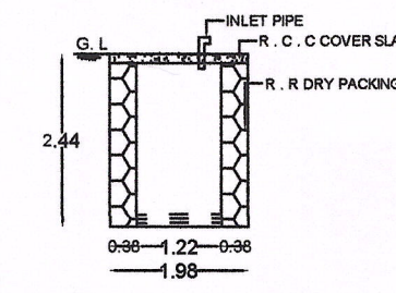
RAIN WATER STORAGE TANK SECTION
