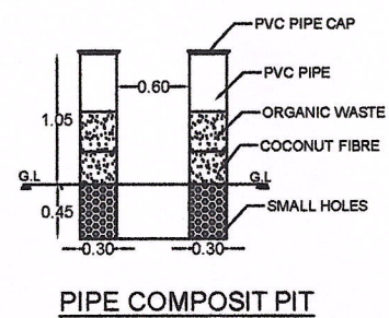
PIPE COMPOSITE PIT
