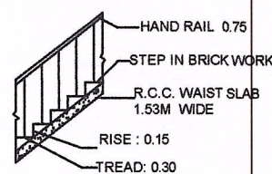
STAIR CASE SECTION
