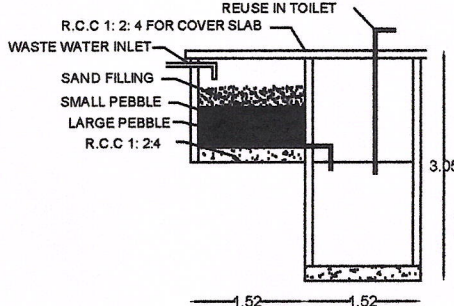
RECYCLING OF WASTE WATER
