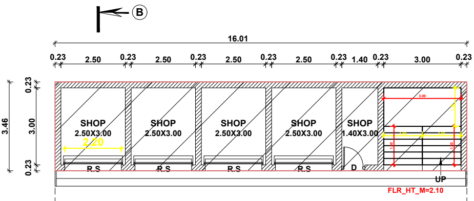
EXISTING GROUND FLOOR PLAN DOOR NOS: II-7-15, II-7-15(4), II-7-15(5), II-7-15(6)
