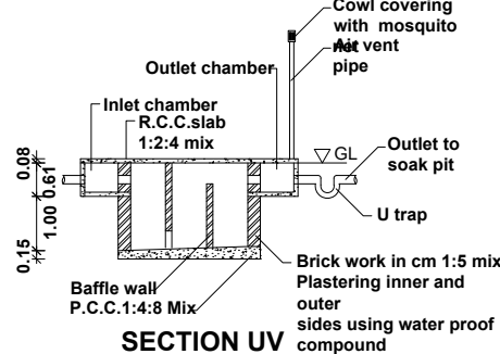
SECTION UV
