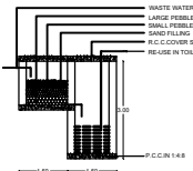
RECYCLING OF WASTE WATER FROM BATH
