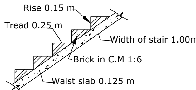
STAIR DETAILS
