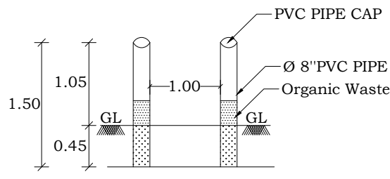
PIPE COMPOSED SYSTEM
