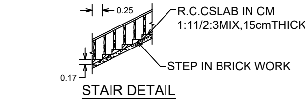
STAIR DETAIL
