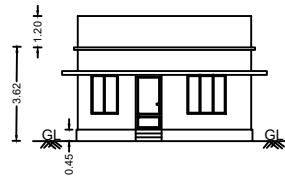
FRONT ELEVATION
