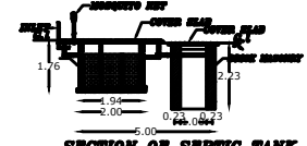
SECTION OF SEPTIC TANK
