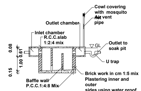
SECTION UV sl cc
