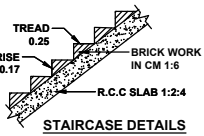
STAIRCASE DETAILS
