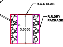
SECTION OF SOAKPIT
