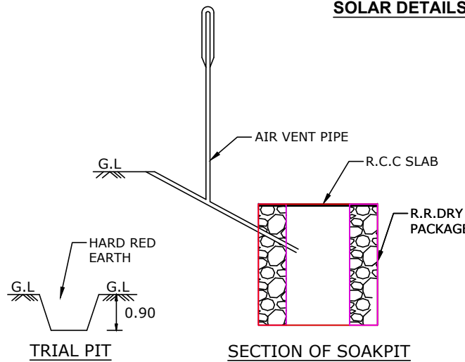
SECTION OF SOAKPIT
