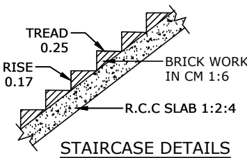
STAIRCASE DETAILS
