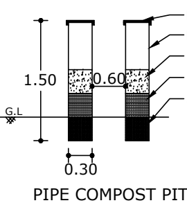
PIPE COMPOST PIT
