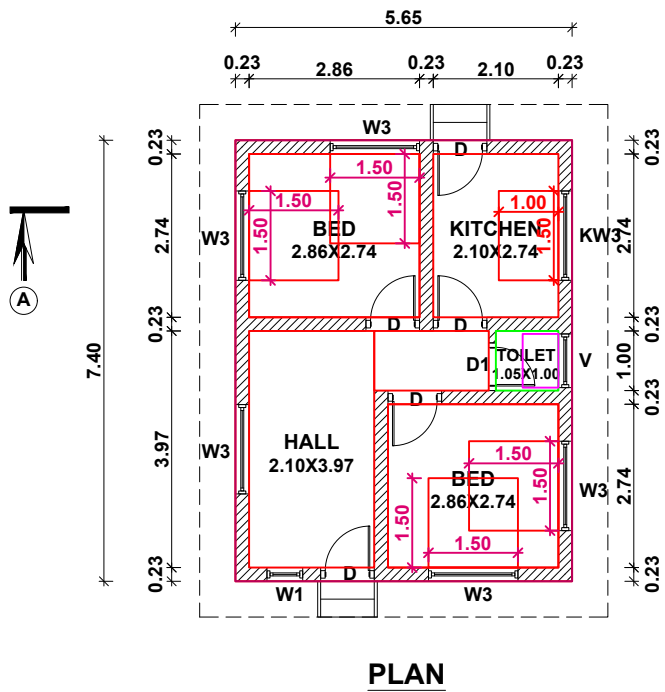
PLAN
