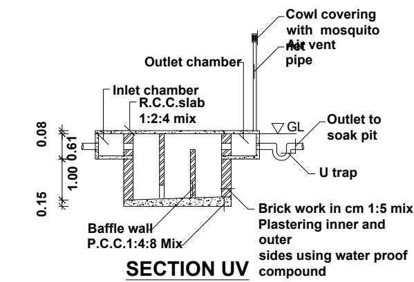
SECTION UV
