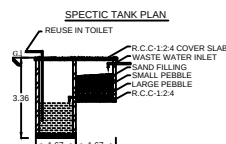
SPECIFIC TANK PLAN RECYCLING OF WASTE WATER KITCHEN & BATH ROOM
