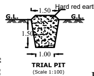
TRIAL PIT (Scale 1:100)
