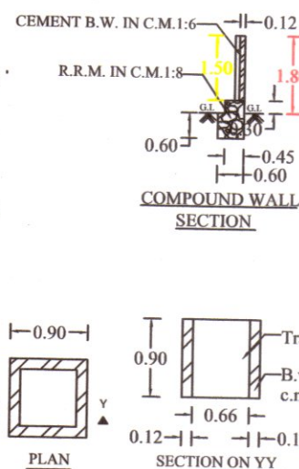
WASTE TRASH PIT
