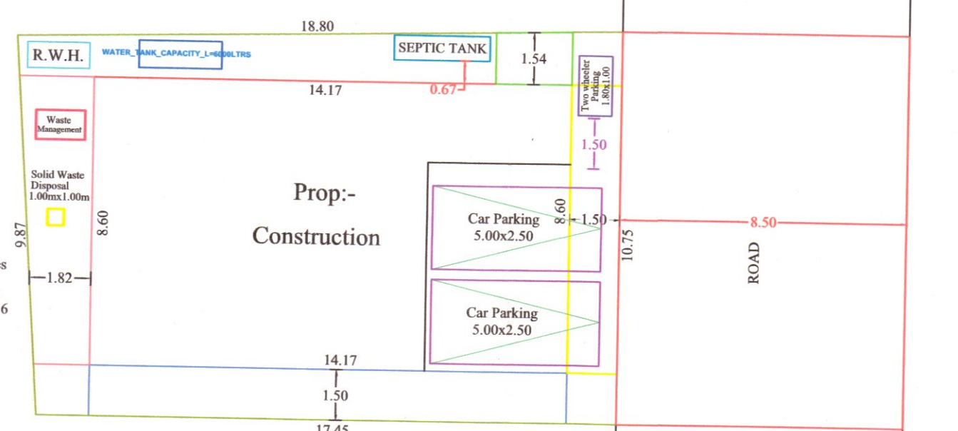
SITE PLAN
