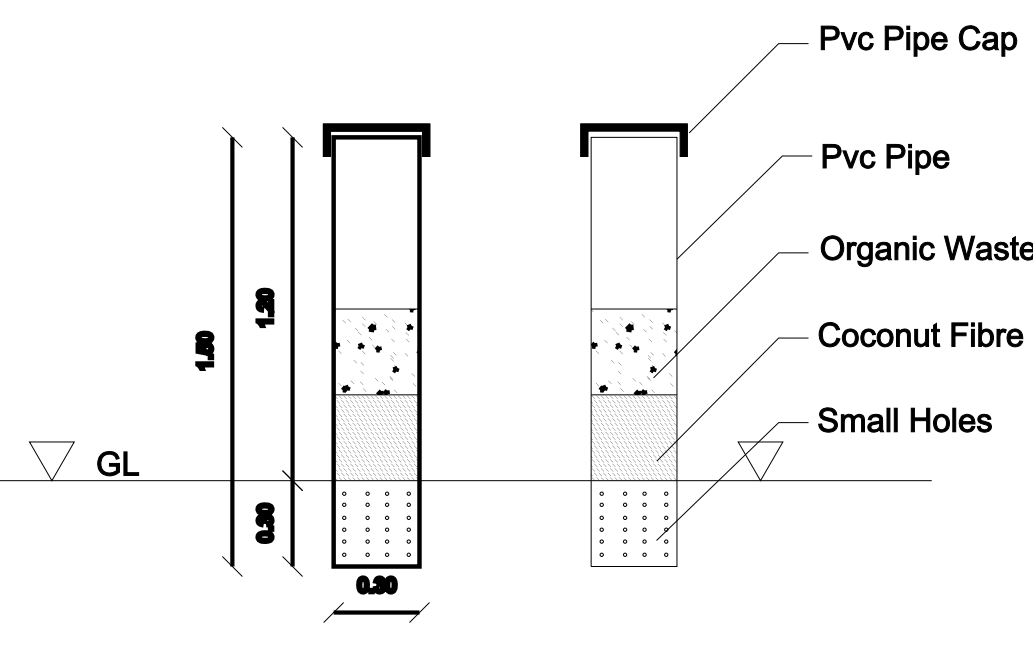
PIPE COMPOST PIT
