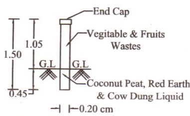
PIPE COMPOSTER
