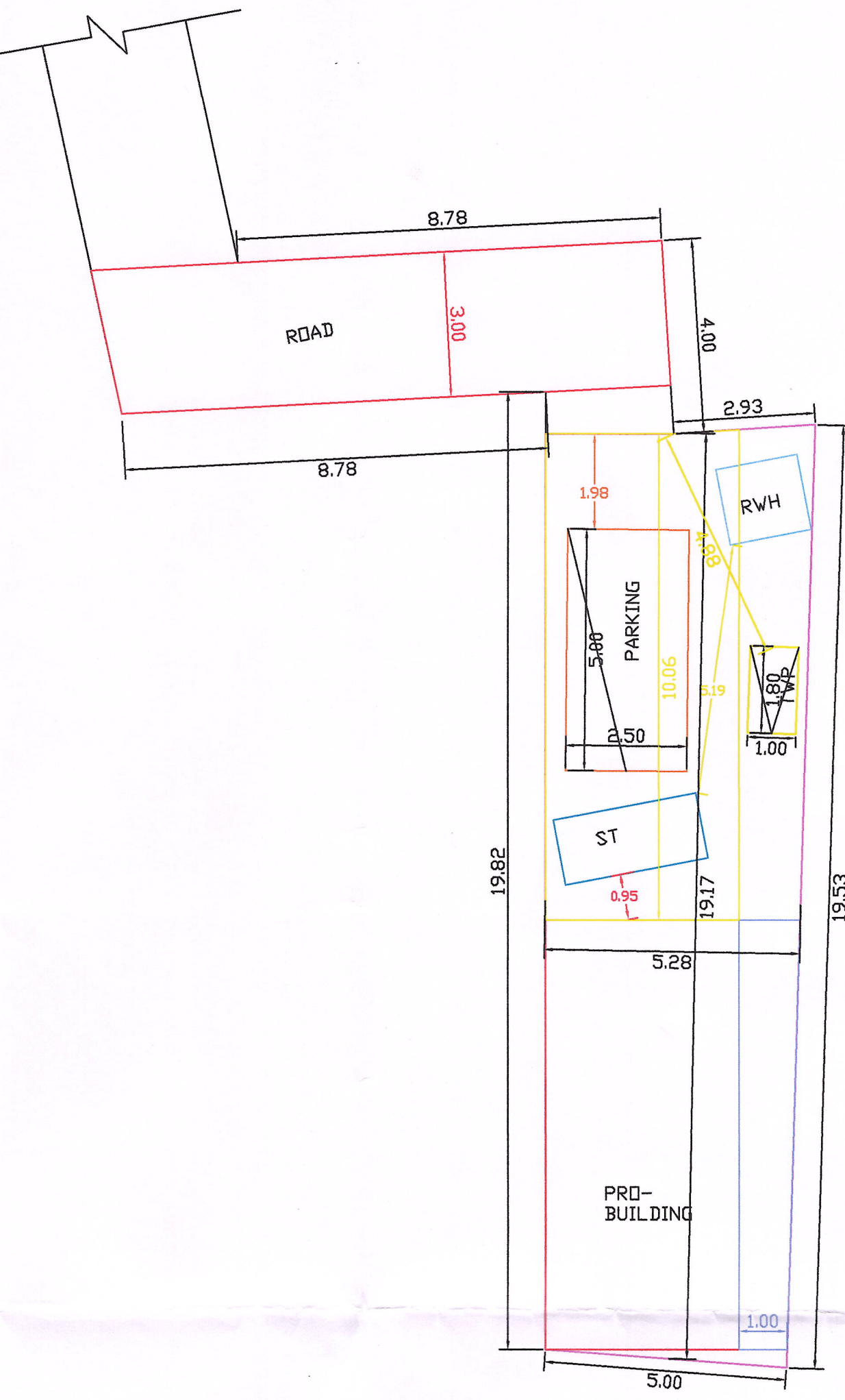
SITE PLAN [1:100]
