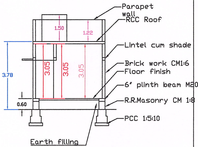
SECTION ON A-A [1:100]
