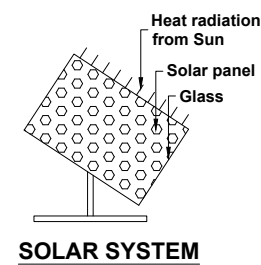
SOLAR SYSTEM
