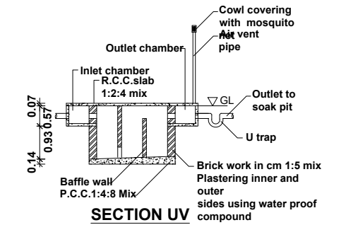
SECTION UV
