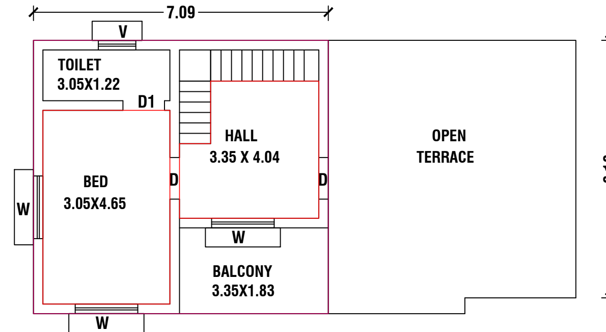
GROUND FLOOR PLAN SCALE 1:100 ALL DIMENSIONS ARE IN "METRE"
