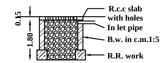
PIPE COMPOST PIT
