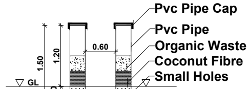
PIPE COMPOST PIT
