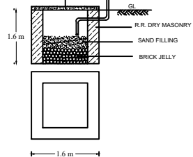
RAINWATER HARVESTING DETAILS
