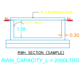
RWTH SECTION (SAMPLE)
