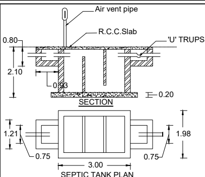
SEPTIC TANK PLAN
