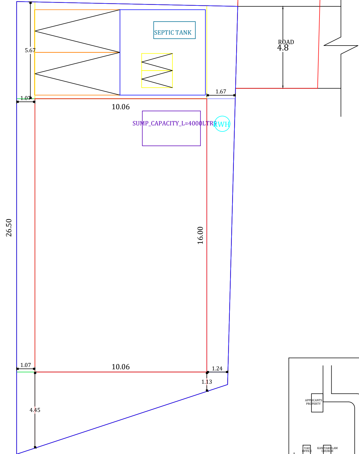
SITE PLAN
