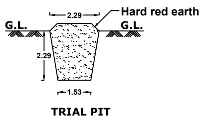
TRIAL PIT
