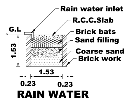
RAIN WATER HARVESTING PIT
