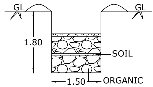
COMPOST PIT
