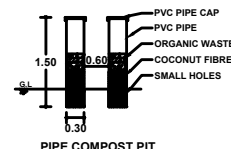
PIPE COMPOST PIT
