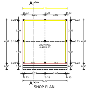
SHOP PLAN
