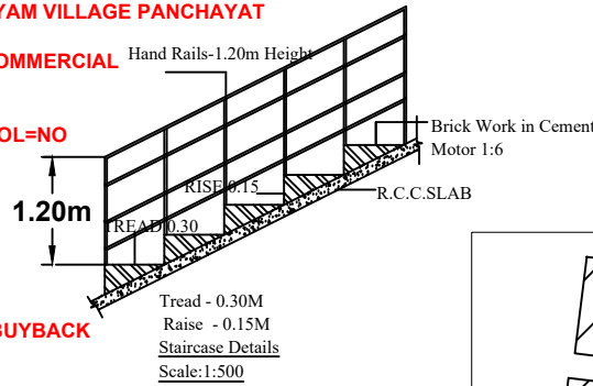
Staircase Details
