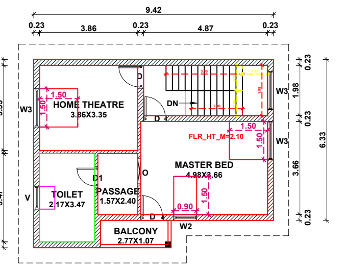
PRO.SECOND FLOOR PLAN
