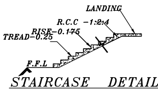
STAIRCASE DETAIL
