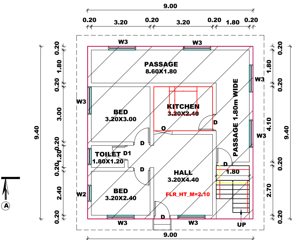
EX.GROUND FLOOR PLAN DOOR NO:5-112B
