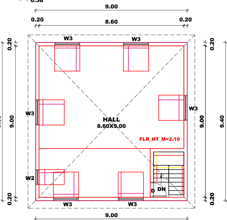
FIRST FLOOR PLAN EXISTING & EXTENSION
