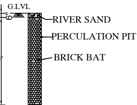
PERCOLATION PIT
