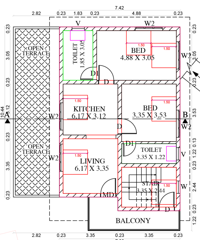
FIRST FLOOR HOUSE-2
