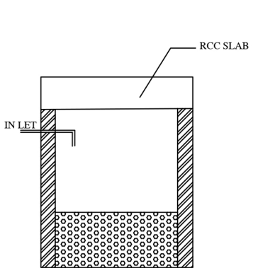
RECYCLING OF WASTE WATER
