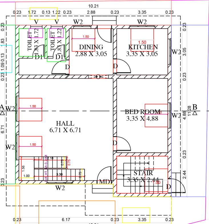
GROUND FLOOR HOUSE-1
