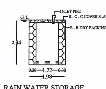
RAIN WATER STORAGE TANK SECTION
