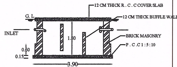
SECTION ON B-B
