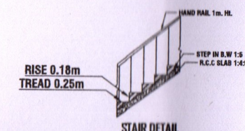
STAIR DETAIL
