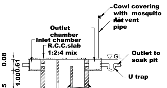
SECTION UV
