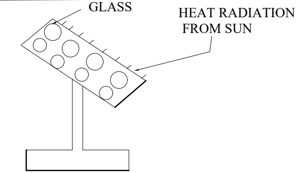
SOLAR SYSTEM
