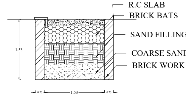
RAIN WATER HARVESTING TANK
