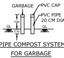
PIPE COMPOST SYSTEM FOR GARBAGE
