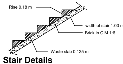
Stair Details
