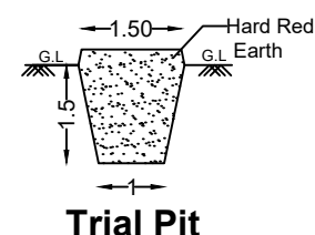
Trial Pit
