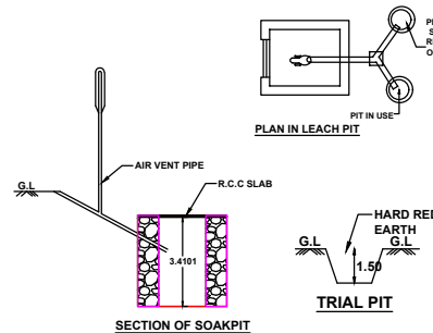
SECTION OF SOAK PIT
