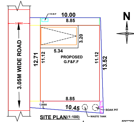
SITE PLAN (1:100)
