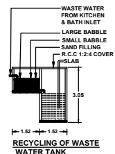
RECYCLING OF WASTE WATER TANK
