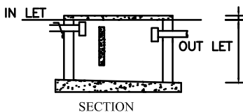
SEPTIC TANK
