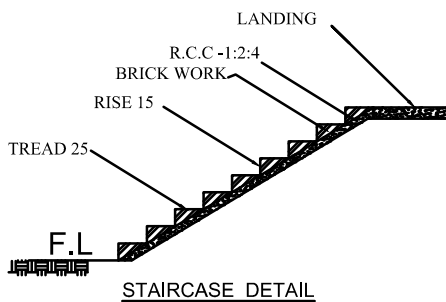
STAIRCASE DETAIL
