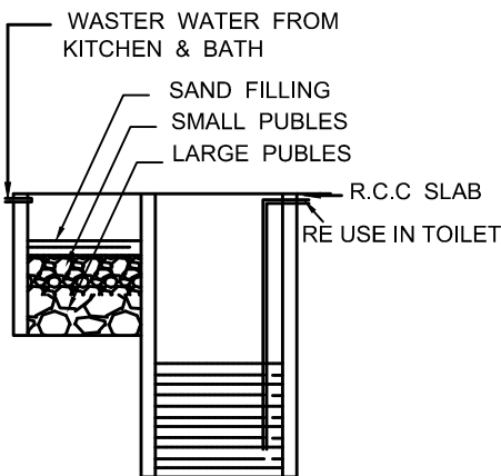
RECYCLING OF WASTE WATER KITCHEN & BATH ROOM
