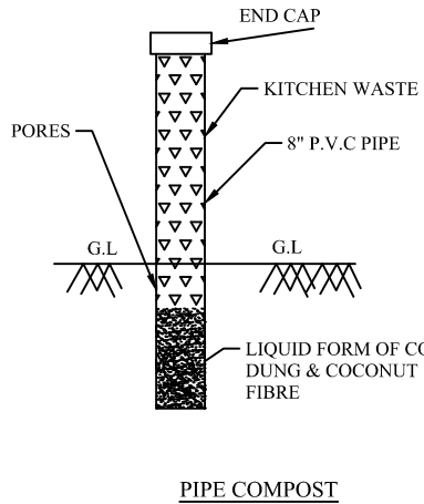
PIPE COMPOST
