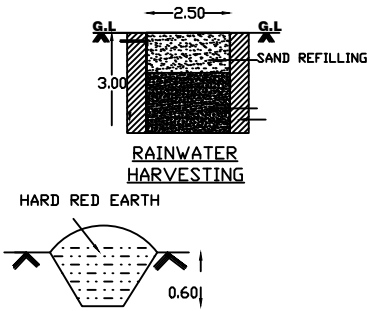
RAINWATER HARVESTING
