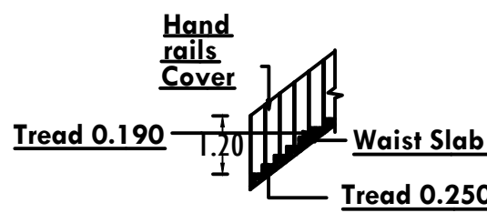
STAIRCASE DETAILS
