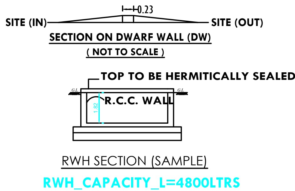
RWH SECTION (SAMPLE)
